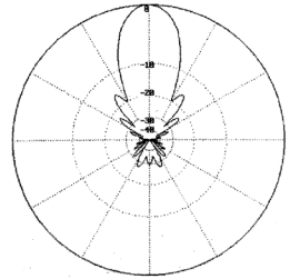
Figure 4C 17-element yagi
